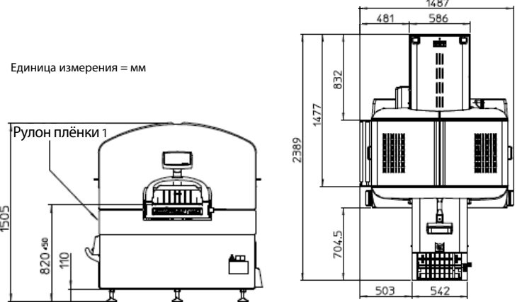
AUTOMAC 40 ZS - In line
